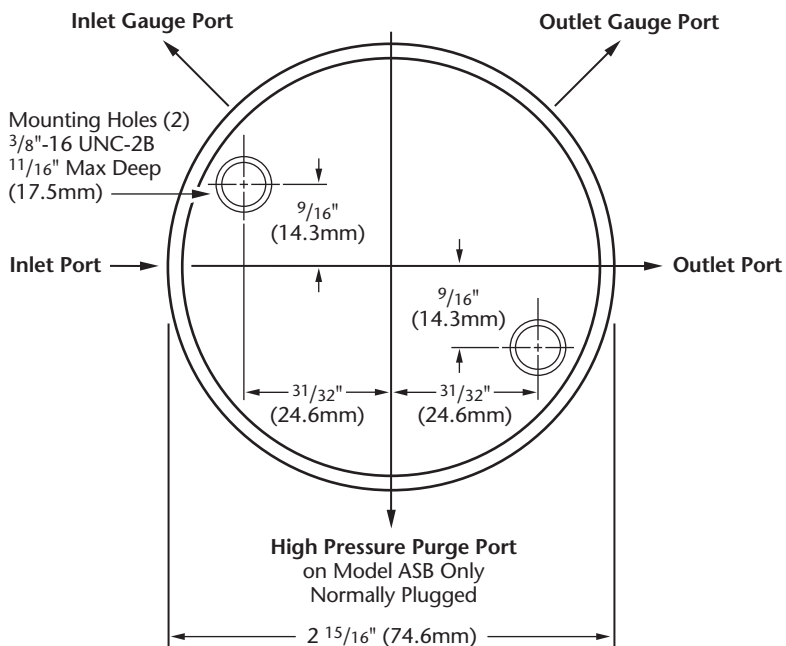
Figure 2 - Models ASB and CRH Regulators Rear View Body Dimensions for Mounting to Bracket or Panel
