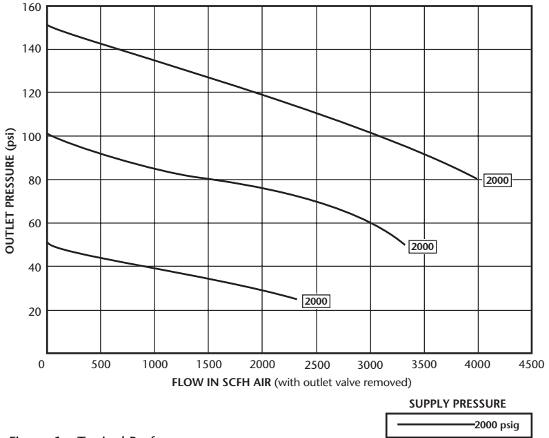
Figure 1 - Typical Performance Models ASB & CRH Regulators
