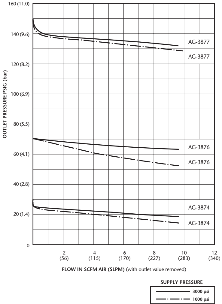
Figure 1 – Typical Performance AG3870 Series
