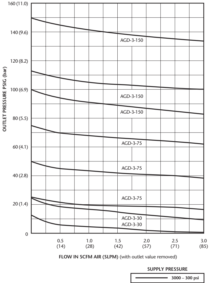
Figure 2 – Typical Performance AGD Series
