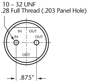
Figure 3 – Model AG3870 Series All Dimensions are Reference Only
